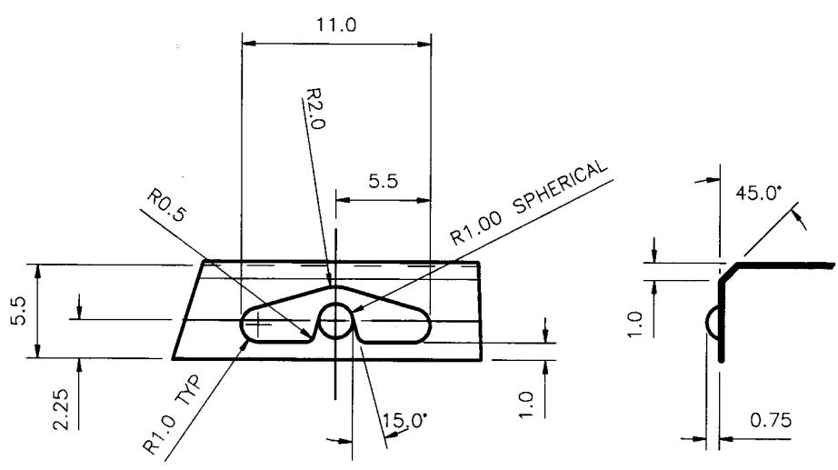
DETAIL A @ 4:1 10 POSITIONS
