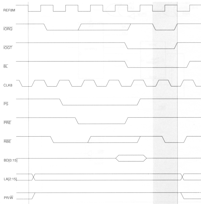
Figure 7: Stretched expansion card read cycle
