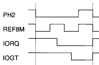
Figure 19: Fast I/O cycle
