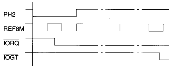
Figure 18: I/O cycle
