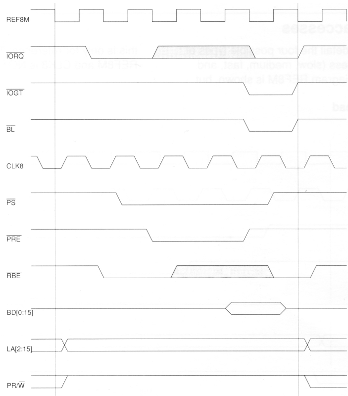
Figure 6: IOC driving an expansion card read cycle
