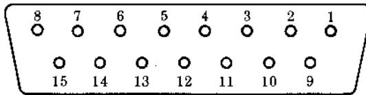
Figure 3 The 'analogue in' socket (viewed from outside case)
