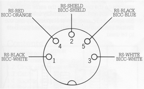
Figure 2: DIN pin number allocations
